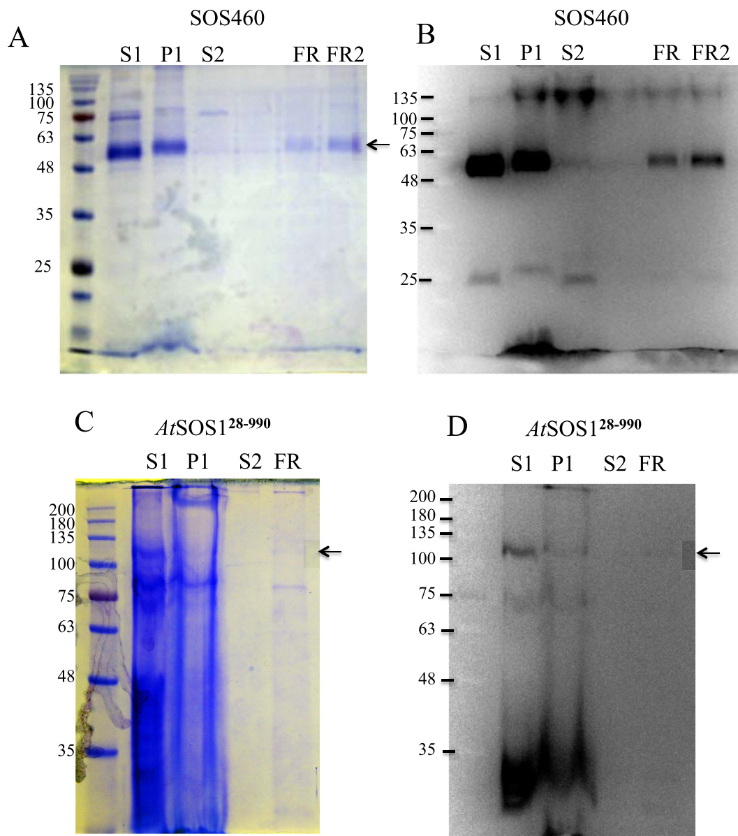
Fig. 5. Analysis of reconstituted SOS460 (A, B) and SOS990 (C, D) proteins by SDS-PAGE. Enriched SOS1 proteins were used after purification via immobilized metal affinity chromatography and size fractionation. Reconstitution into soy asolectin is shown, S1 = Starting protein solution, P1 = pellet from the first 10,000 \times g containing protein (in the presence of 5 mM MgCl_2 ) and lipid not solubilized and precipitated. S2, supernatant of 265,000 \times g spin. FR, final pellet after 265,000 \times g spin containing asolectin-protein vesicles. FR2, enriched fraction asolectin-protein vesicles.
